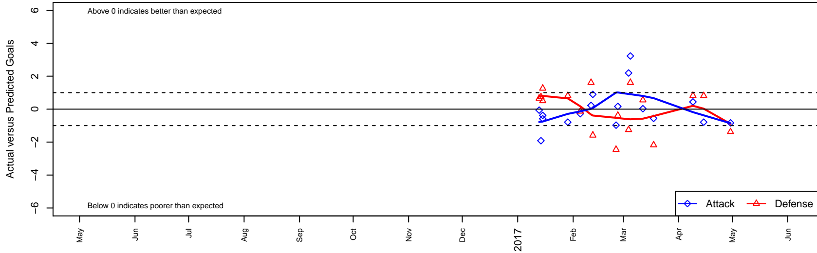
GPS Newberg B99 Dots are actual minus expected GF (blue circles) and GA (red triangles). Blue line is smoothed change in attack strength. Red is smoothed change in defense strength.
